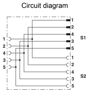
Contact assignment of the M12 Y distributor
