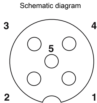
Pin assignment M12 socket, 5-pos., A-coded, socket side view
