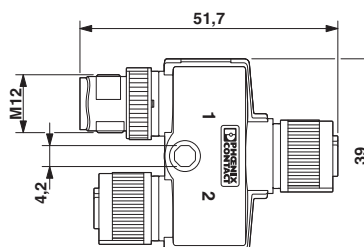
Dimensional drawing
