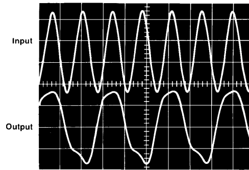
700 MHz Operation
