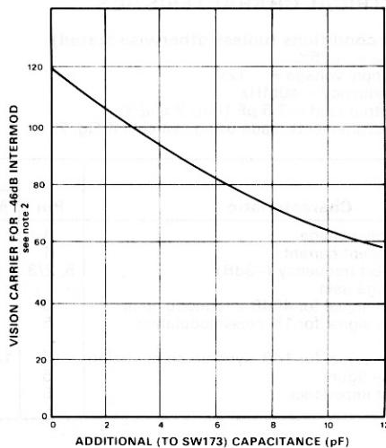
Fig. 7 Intermodulation performance v. load capacitance (see note 2)
