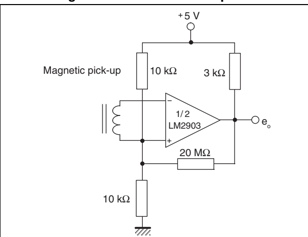
Figure 13. Transducer amplifier
