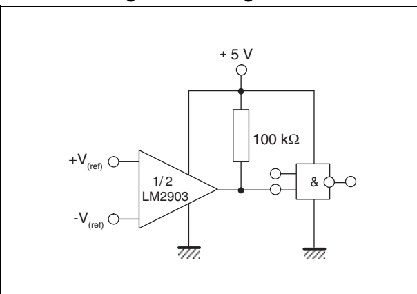
Figure 9. Driving CMOS
