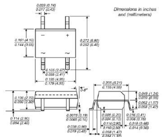
TO-269AA (MBS)
