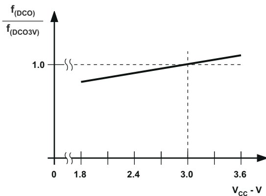
图 8-15. DCO Frequency vs Supply Voltage V CC and vs Ambient Temperature
