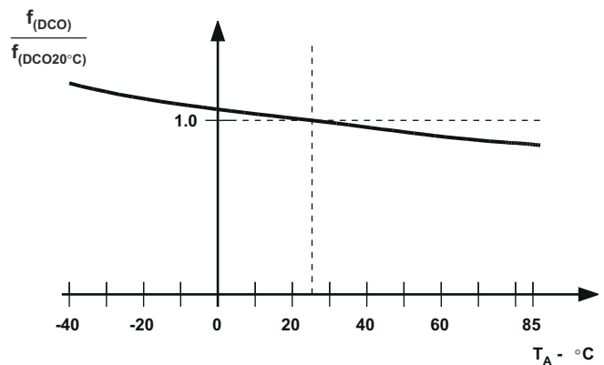
图 8-15. DCO Frequency vs Supply Voltage V CC and vs Ambient Temperature
