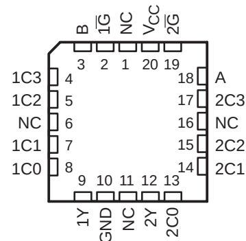
SN54ALS352 . . . FK PACKAGE (TOP VIEW)
