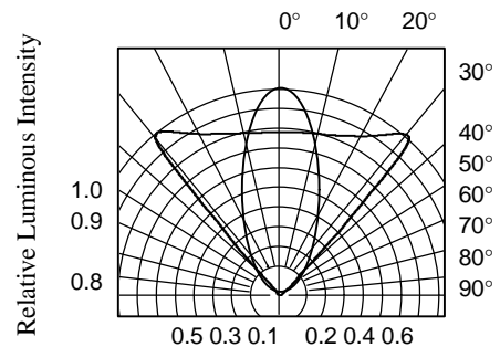
FIG.6 RADIATION DIAGRAM
