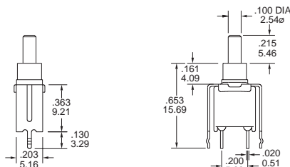
ES-21-CR-A5S (std.) snap-in type
