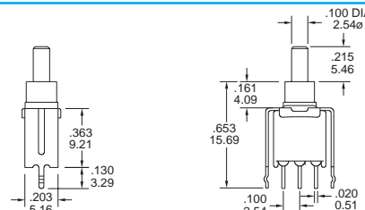
ES-22-CR-A5S (std.) snap-in type
