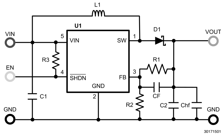
FIGURE 3. LMR64010 Demo Board Schematic
