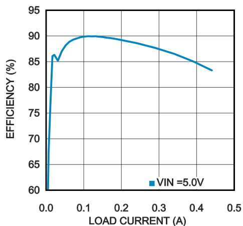
Efficiency vs. Load Current LMR62014, V_{OUT} = 12V
