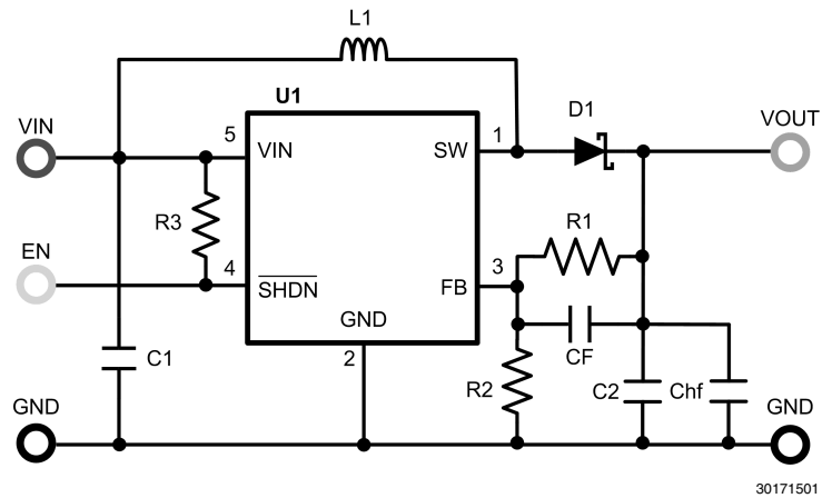
FIGURE 2. LMR62014 Demo Board Schematic
