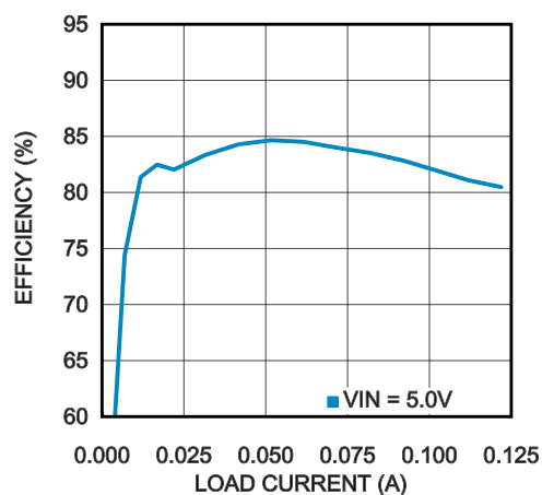
Efficiency vs. Load Current LMR64010, V_{OUT} = 24V
