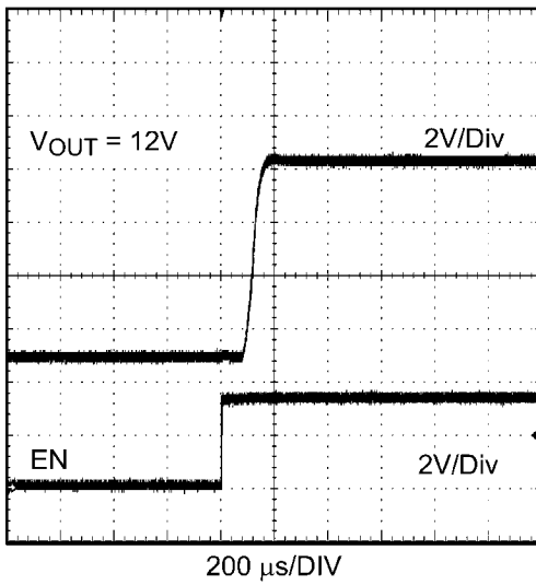
Startup Waveform
