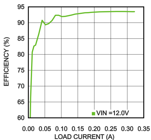
Efficiency vs. Load Current LMR64010, V_{OUT} = 24V
