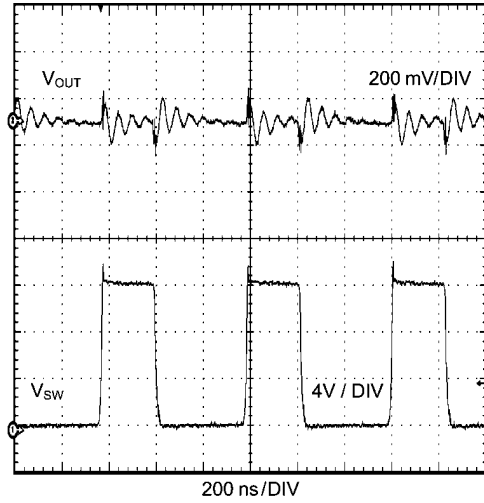
Switching Node and Output Voltage Waveforms LMR62014
