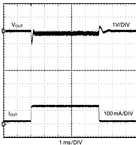
Load Transient Waveforms LMR64010 I_{OUT} = 13 to 125mA
