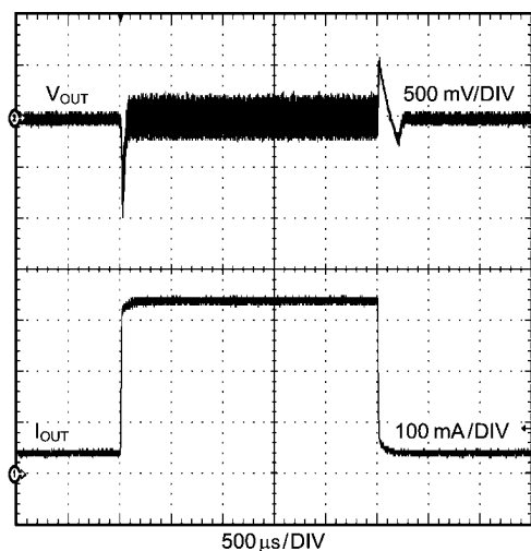
Load Transient Waveforms LMR62014 I_{OUT} = 33 to 330mA
