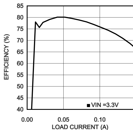
Efficiency vs. Load Current LMR62014, V_{OUT} = 12V
