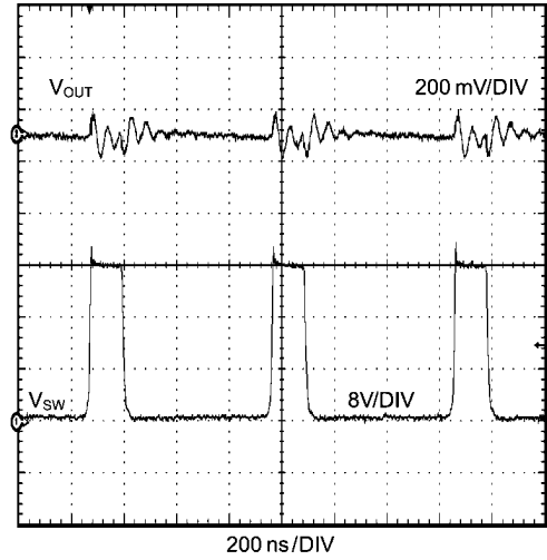
Switching Node and Output Voltage Waveforms LMR64010
