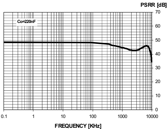
Figure 13. PSRR
