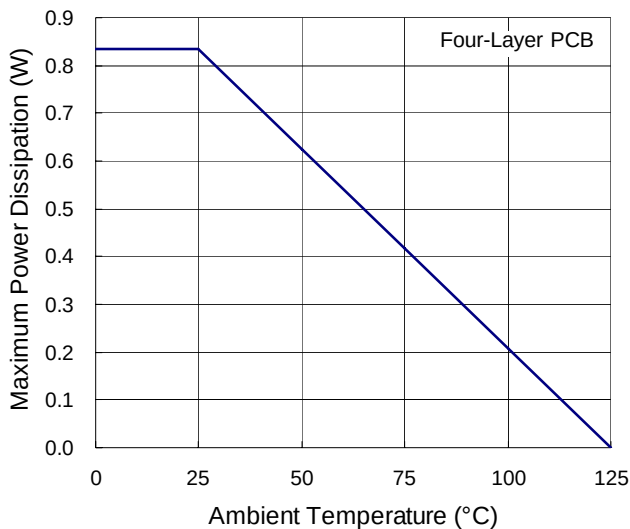
Figure 3. Derating Curve for RT9526A Package
