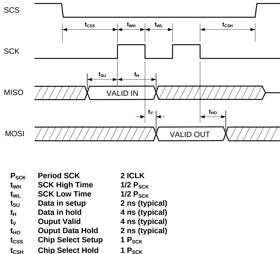
Figure 6-22. SPI Timing Diagram
