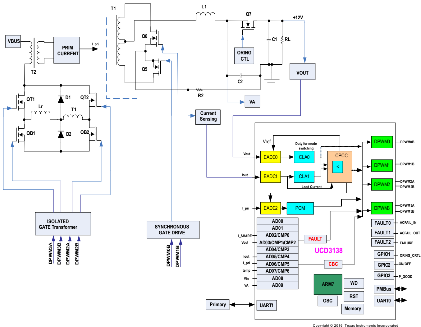
Figure 7-1. Phase-Shifted Full-Bridge
