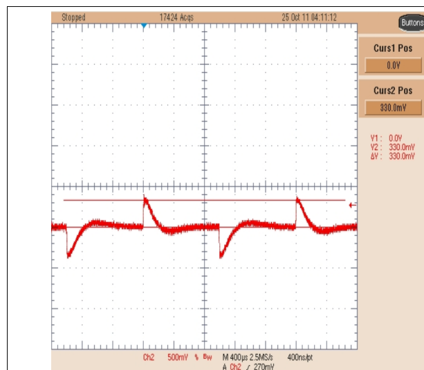
Figure 7-10. Load Transient
