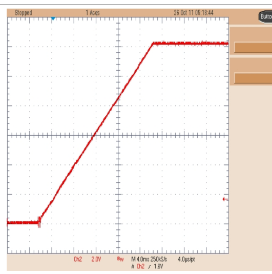
Figure 7-11. V OUT Soft Start
