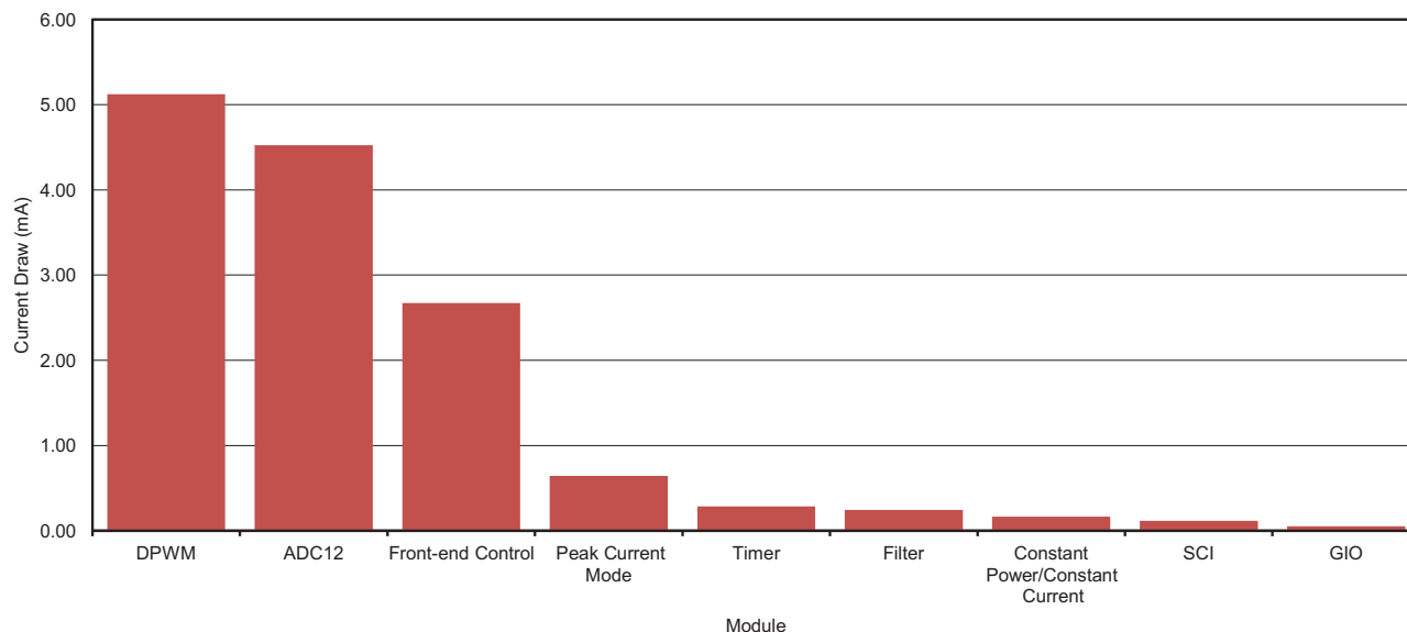
Figure 5-10. Clock Gating Power Savings
