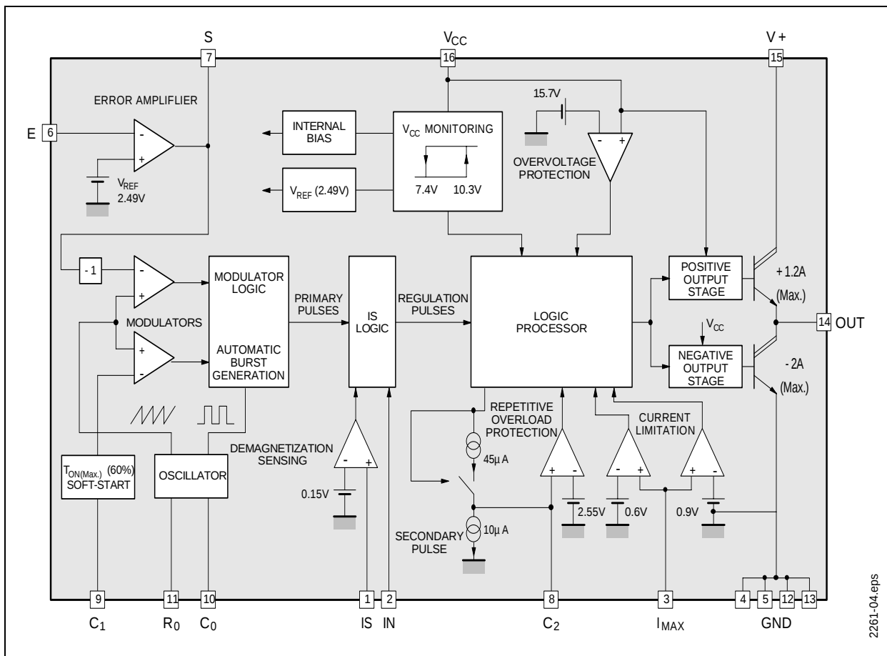
Figure 2. Block Diagram
