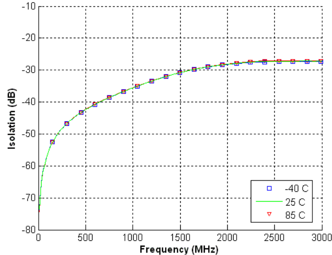
Figure 7. Isolation, Tx-Rx, V_{DD}=3.3V
