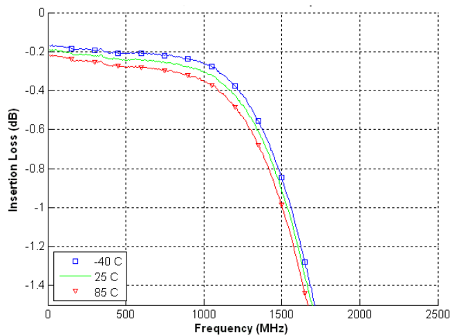
Figure 10. Tx Insertion Loss, V_{DD}=3.3V
