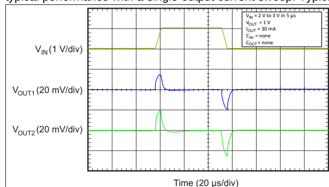
Figure 13. Line Transient
