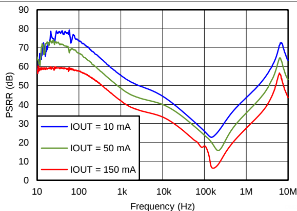
Figure 25. Power-Supply Rejection Ratio vs Frequency ( V_{OUT} = 3.3 V)
