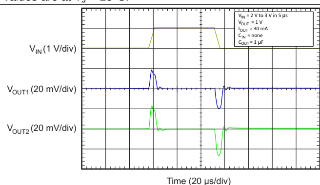
Figure 14. Line Transient
