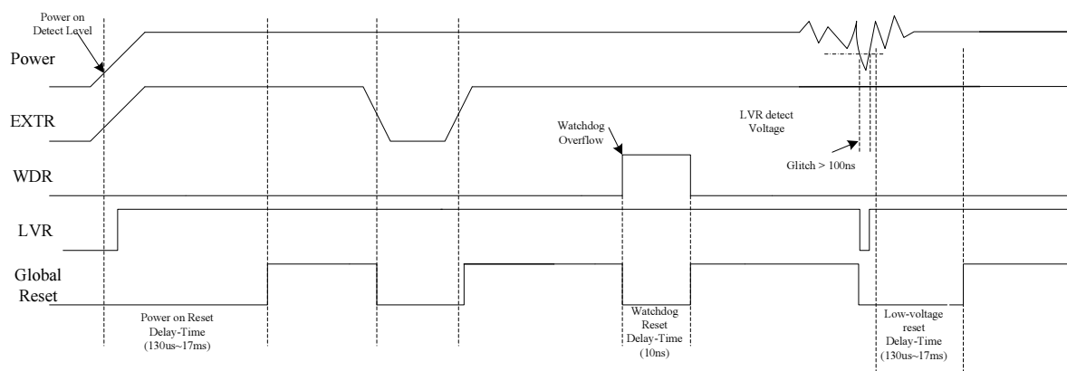
Figure 3.0-2 Global Timing
