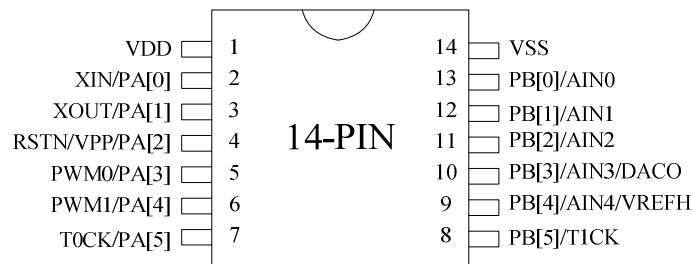
FM8PC71AM-A PDIP/SOP
