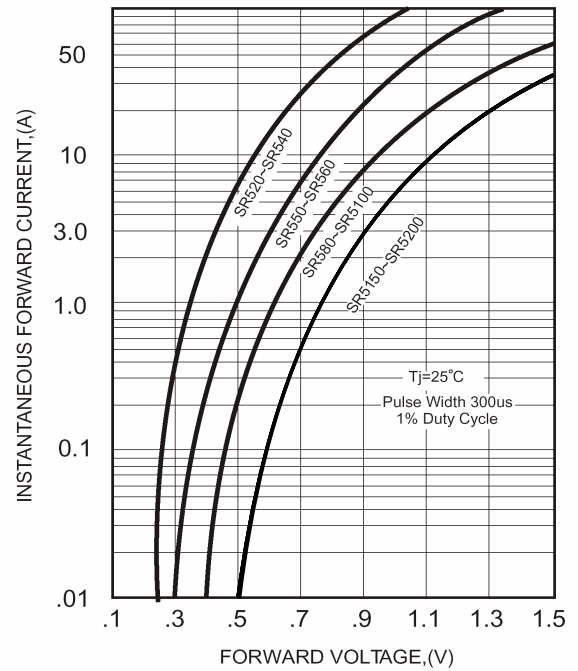
FIG.2-TYPICAL FORWARD CHARACTERISTICS
