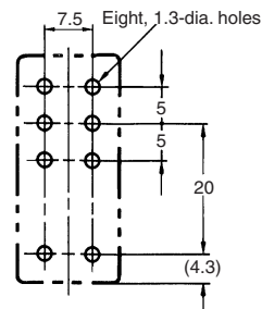
Mounting Holes
