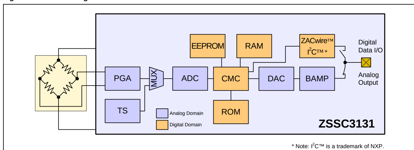
Figure 2.1 Block Diagram of the ZSSC3131
