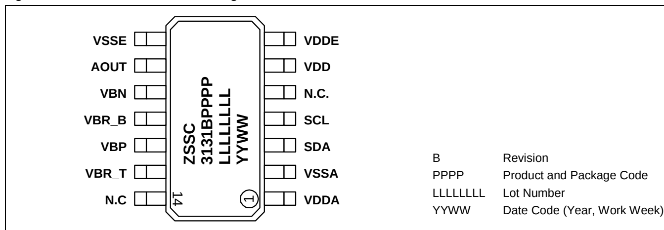
Figure 4.1 ZSSC3131 SSOP14 Pin Diagram
