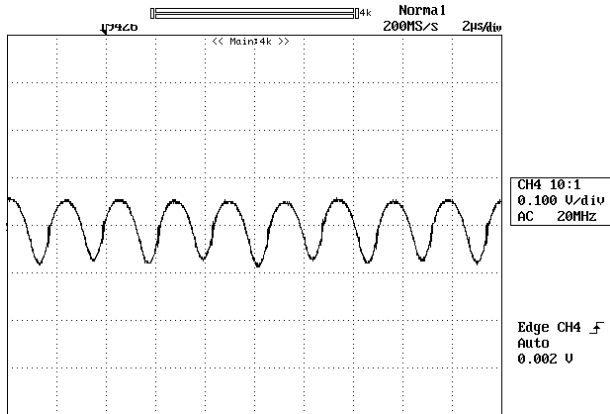
Figure 11: Input Terminal Ripple Current, i_o , at full rated output current and nominal input voltage with 12\mu\text{H} source impedance and 33\mu\text{F} electrolytic capacitor (100mA/div, 2us/div)
