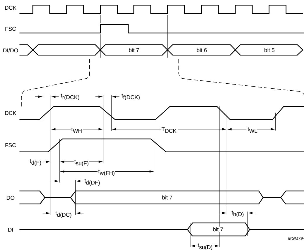
Fig.31 4-wire interface timing in IOM mode.
