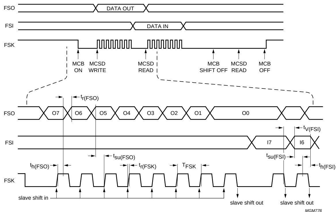
Fig.12 MCB timing for a Microwire compatible device.
