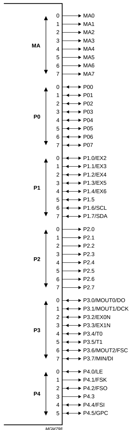
Fig.35 DTAM general purpose digital I/O configuration.
