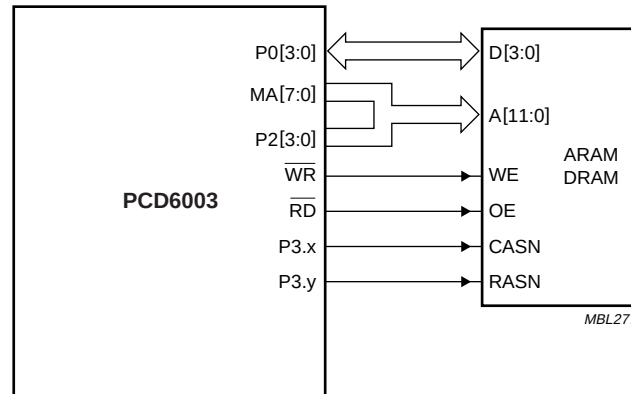
Fig.27 DRAM/ARAM memory connection.
