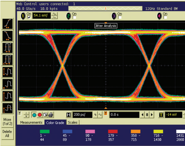
Generate multi-level signals with programmable ISI and jitter up to 6 Gb/s
