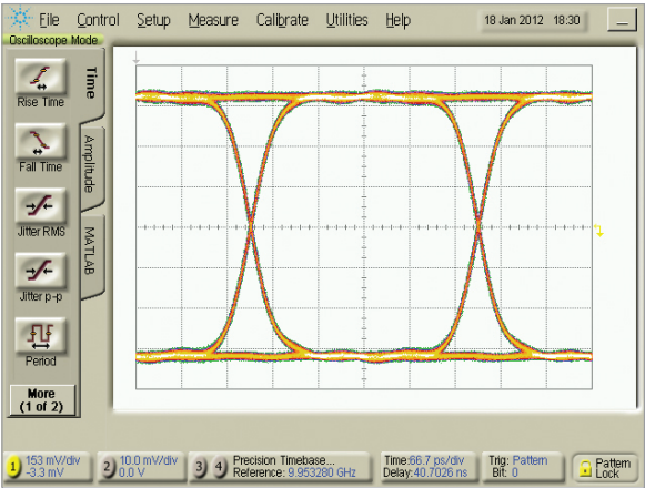
Eye pattern with amplitude 1000 mV with 0 V offset
