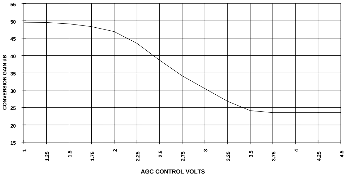
Fig.4 Typical AGC characteristic
