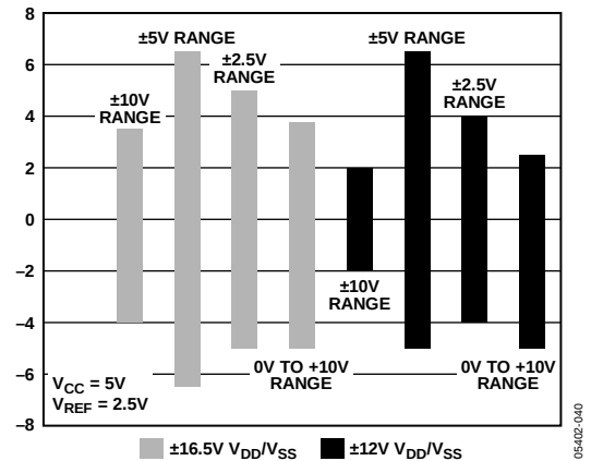
Figure 43. Pseudo Differential Input Range with V_{CC} = 5\text{ V}
