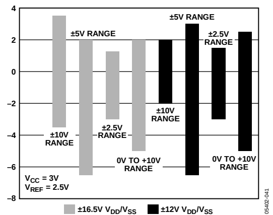
Figure 44. Pseudo Differential Input Range with V_{CC} = 3\text{ V}
