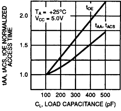
Fig. 10 - NORMALIZED ACCESS TIME vs. LOAD CAPACIYANCE
