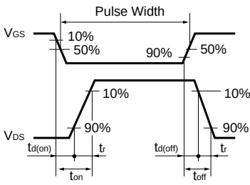
Fig.11 Switching Waveforms
