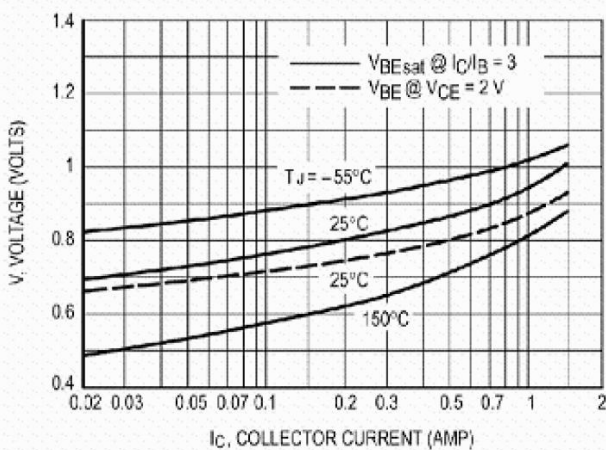
Base-Emitter Voltage
