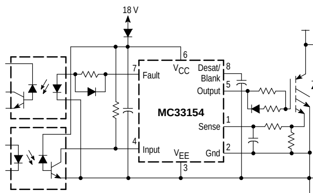
Figure 33. Sense IGBT Application
