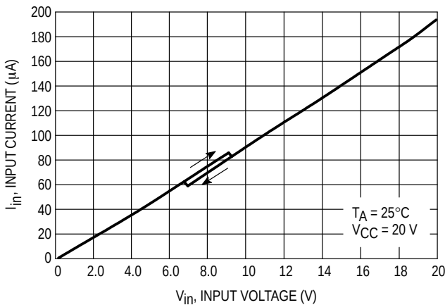
Figure 1. Input Current versus Logic Input Voltage
