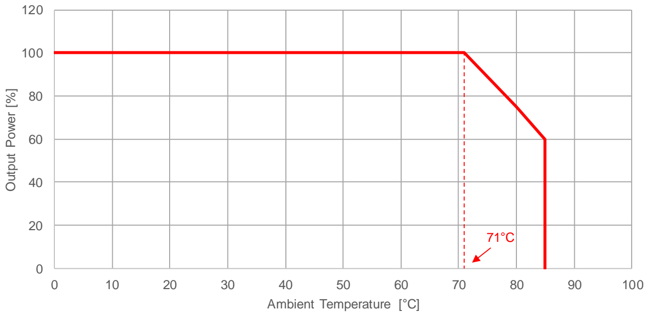
173950x36 Output Power Thermal Derating V_{IN} = 24V , I_{OUT} = 500mA & f_{SW} = 710kHz
