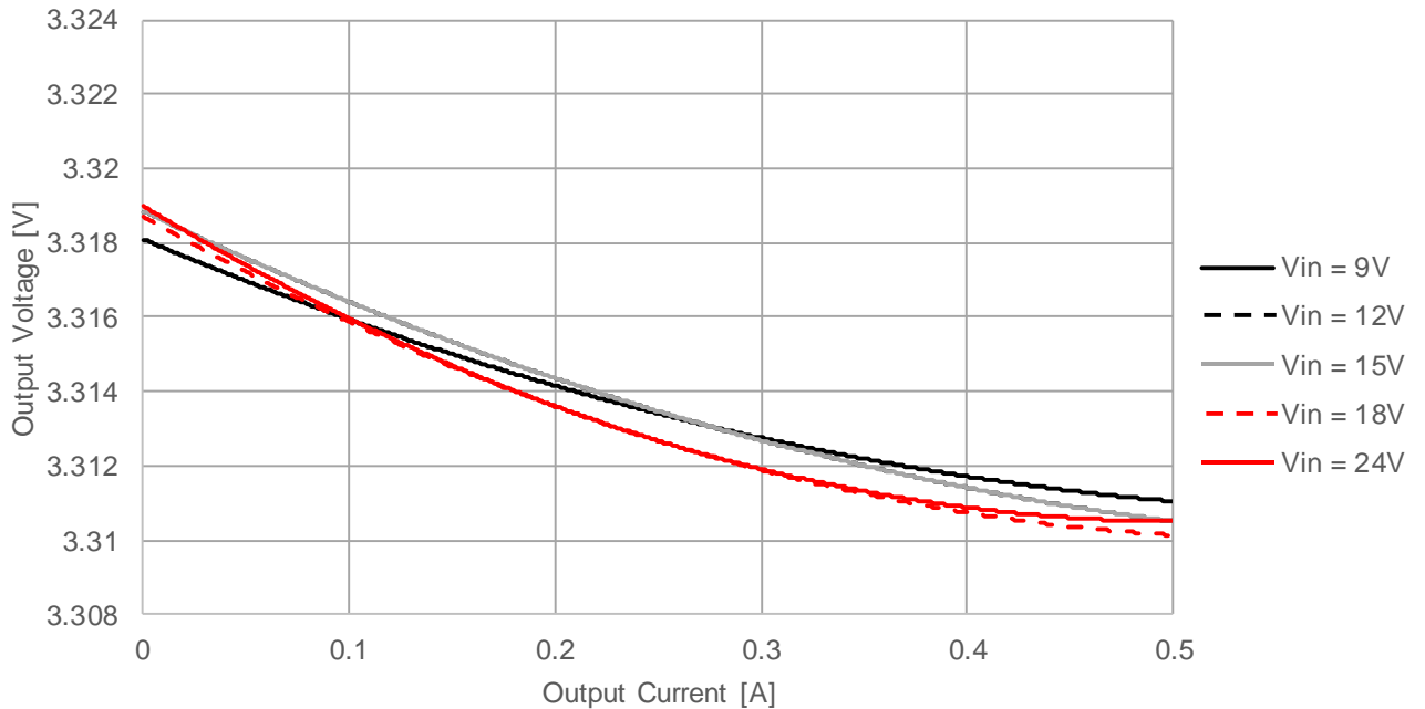
173950336 Load Regulation V_{OUT} = 3.3V , T_A = 85^\circ C
