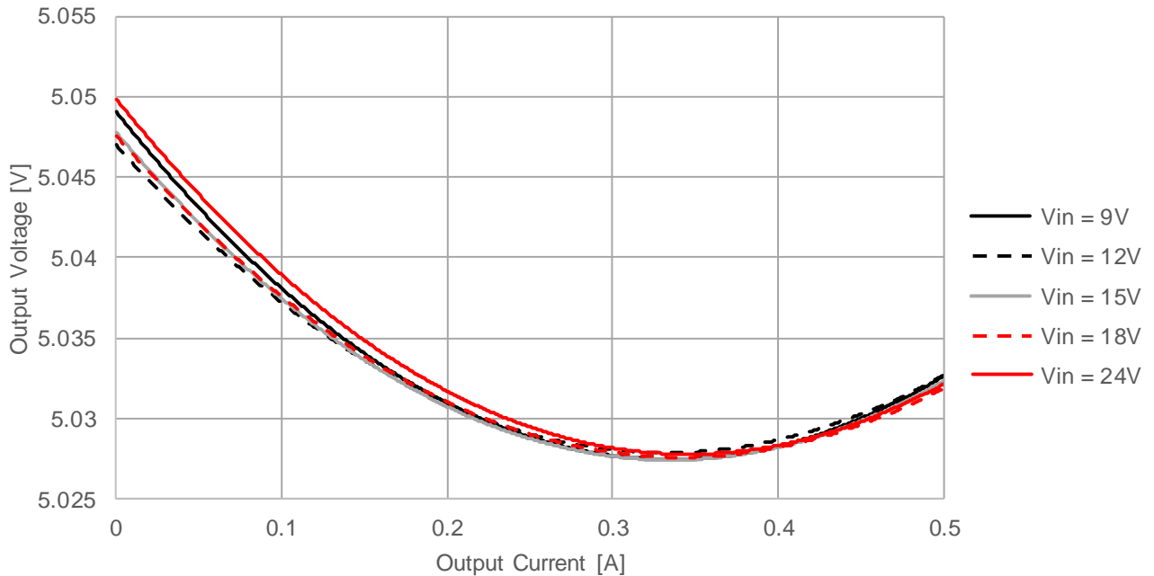
173950536 Load Regulation V_{OUT}=5V, T_A = 85^\circ C
