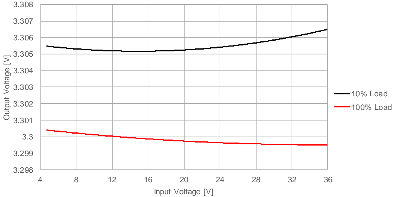
173950336 Line Regulation V_{OUT} = 3.3V , T_A = 25^\circ C
