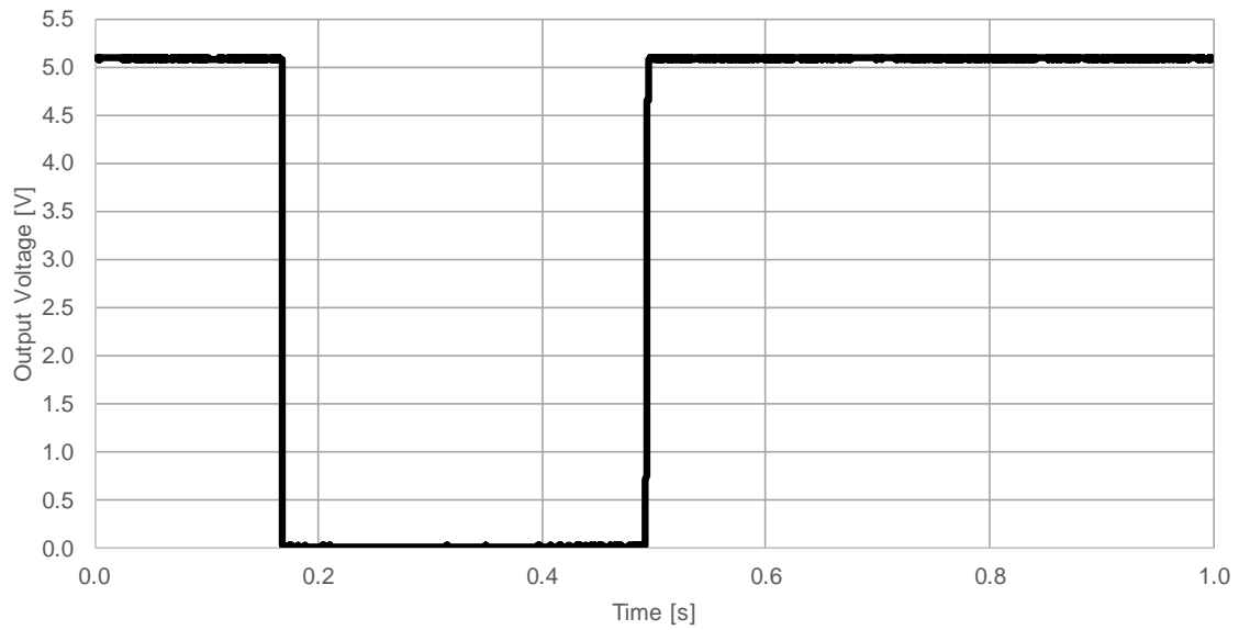
173950536 Short Circuit Protection, V_{IN} = 24V , V_{OUT} = 5V & I_{OUT} = 500mA
