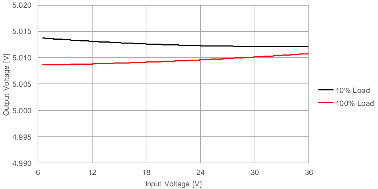
173950536 Line Regulation V_{OUT} = 5V , T_A = 25^{\circ}C
