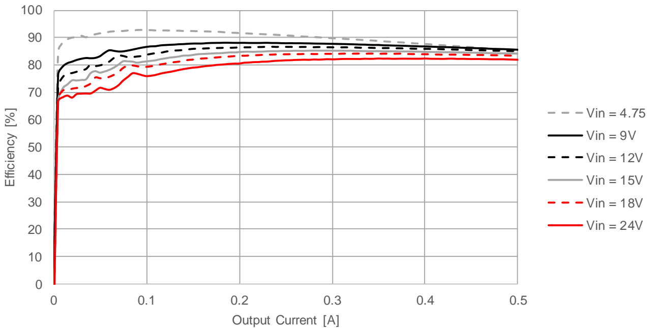
173950336 V_{OUT} = 3.3V , f_{SW} = 710kHz , T_A = 85^\circ C
