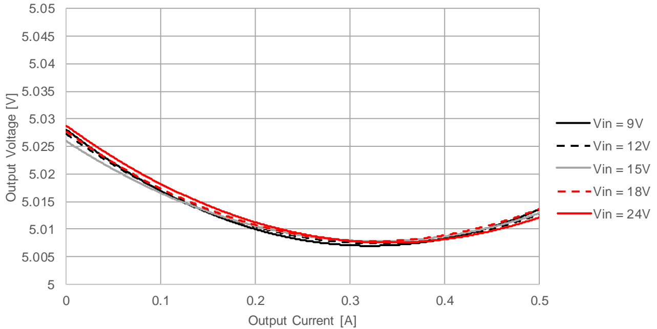
173950536 Load Regulation V_{OUT}=5V, T_A = 25^\circ C
