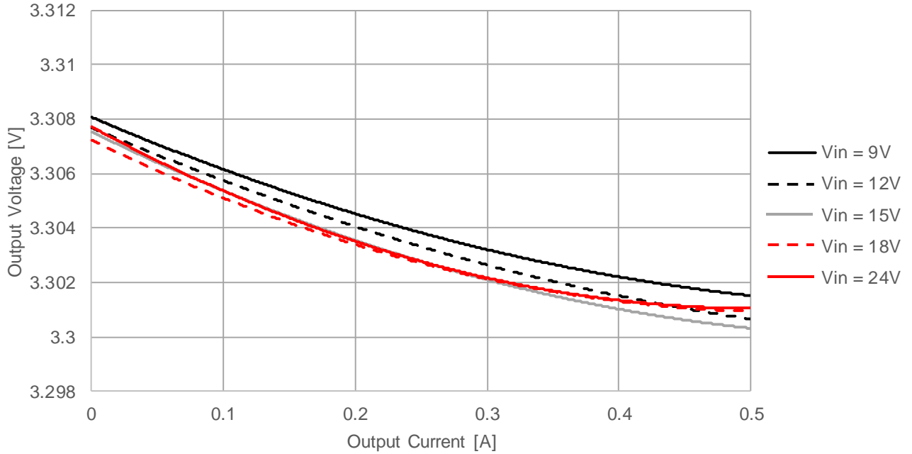
173950336 Load Regulation V_{OUT} = 3.3V , T_A = 25^\circ C
