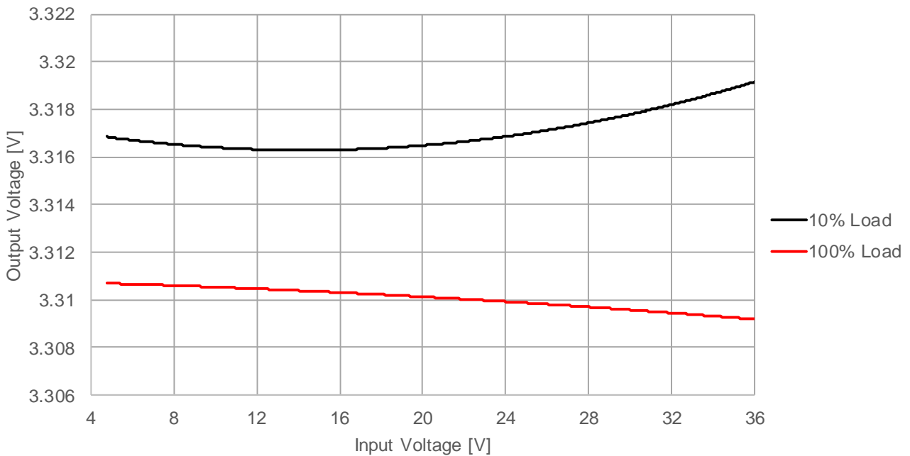
173950336 Line Regulation V_{OUT} = 3.3V , T_A = 85^\circ C
