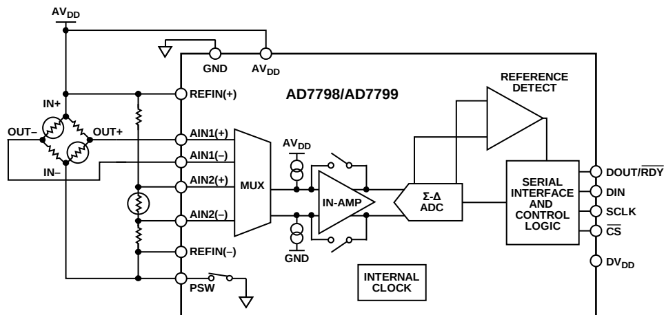
Figure 11. Basic Connection Diagram
