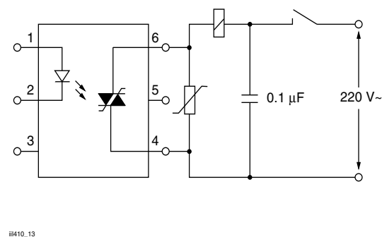
Figure 13. 1- Apply a Capacitor to the Supply Pins at the Load-Side
