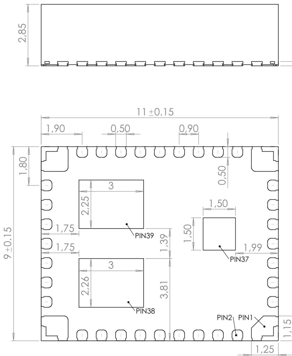
Bottom View
