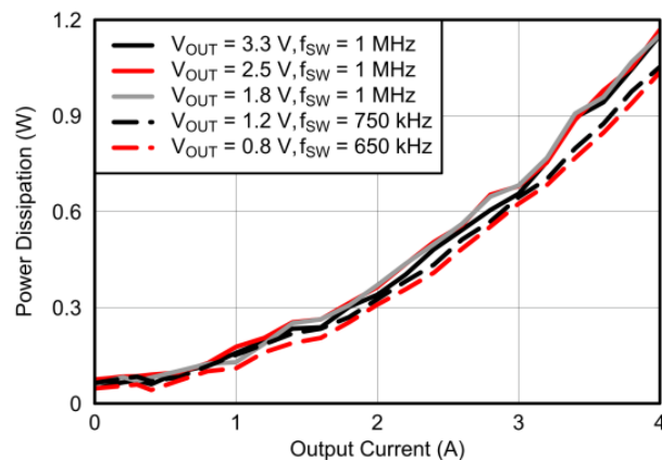
Power Dissipation vs. Output Current
