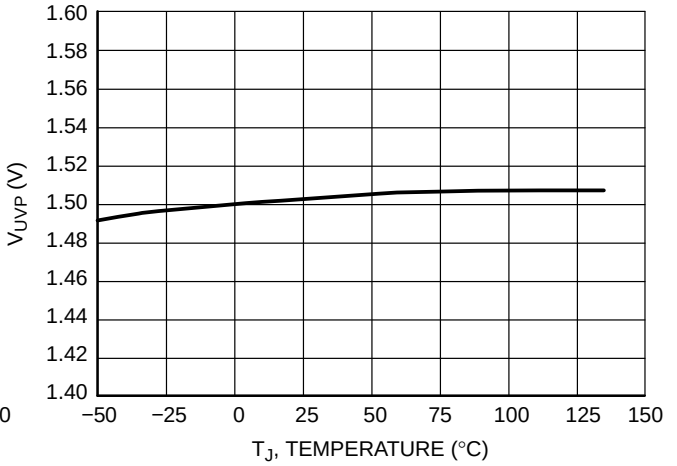
Figure 20. Output Under Voltage Level versus Temperature
