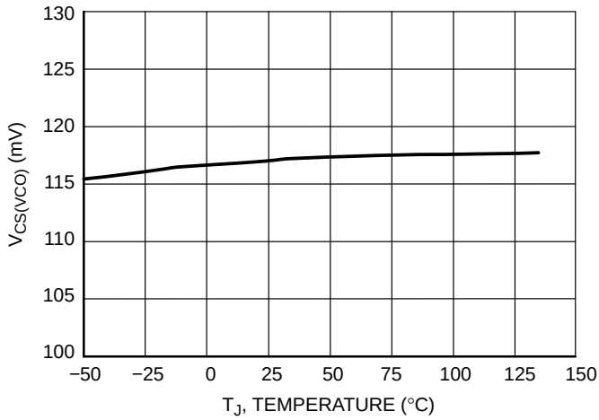
Figure 37. Minimum or Frozen Peak Current on CS Pin versus Temperature
