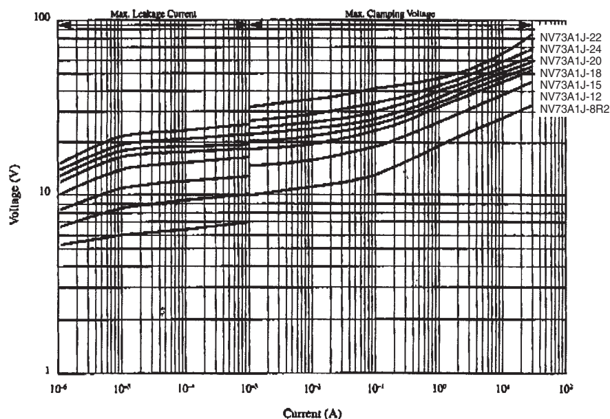
NV73A1J (Ta = +25°C) Voltage-Current Characteristics
