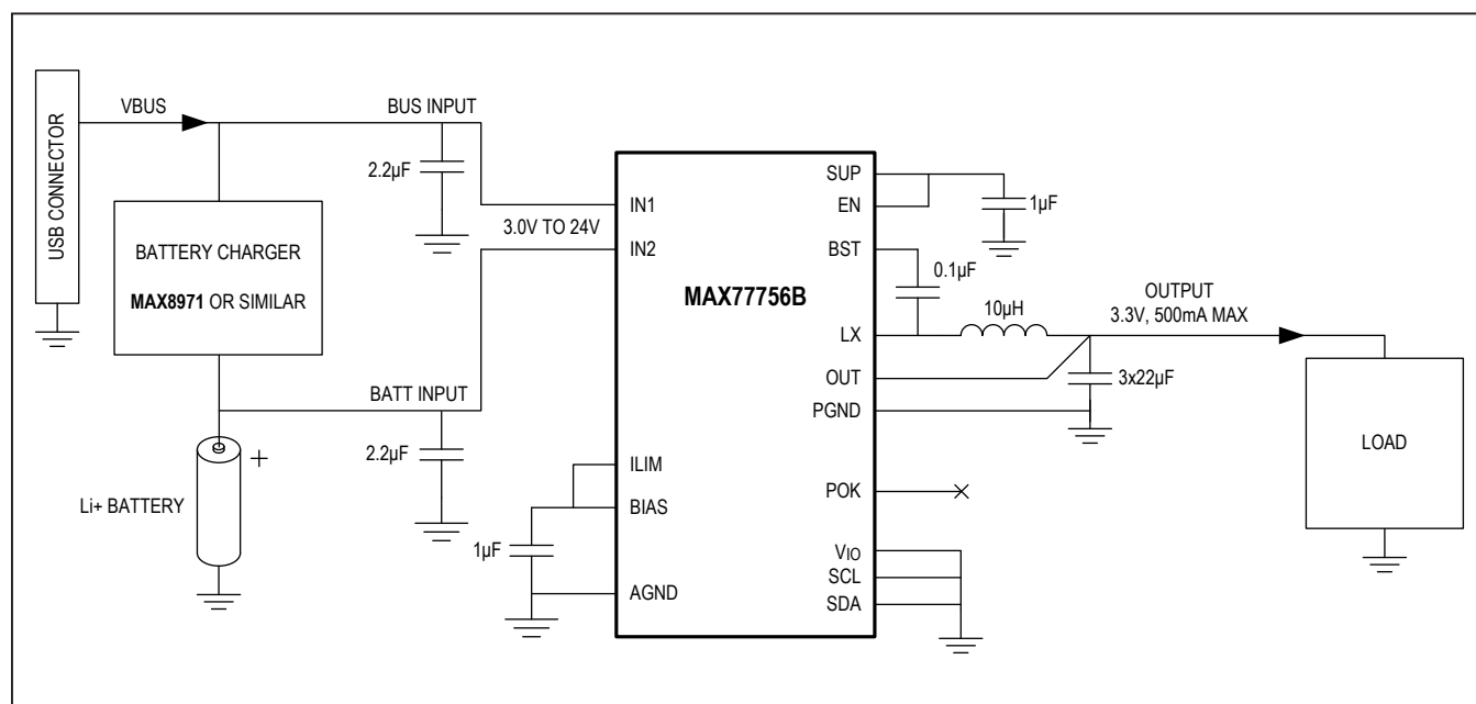
Figure 16. Simple Instant-On Battery System
