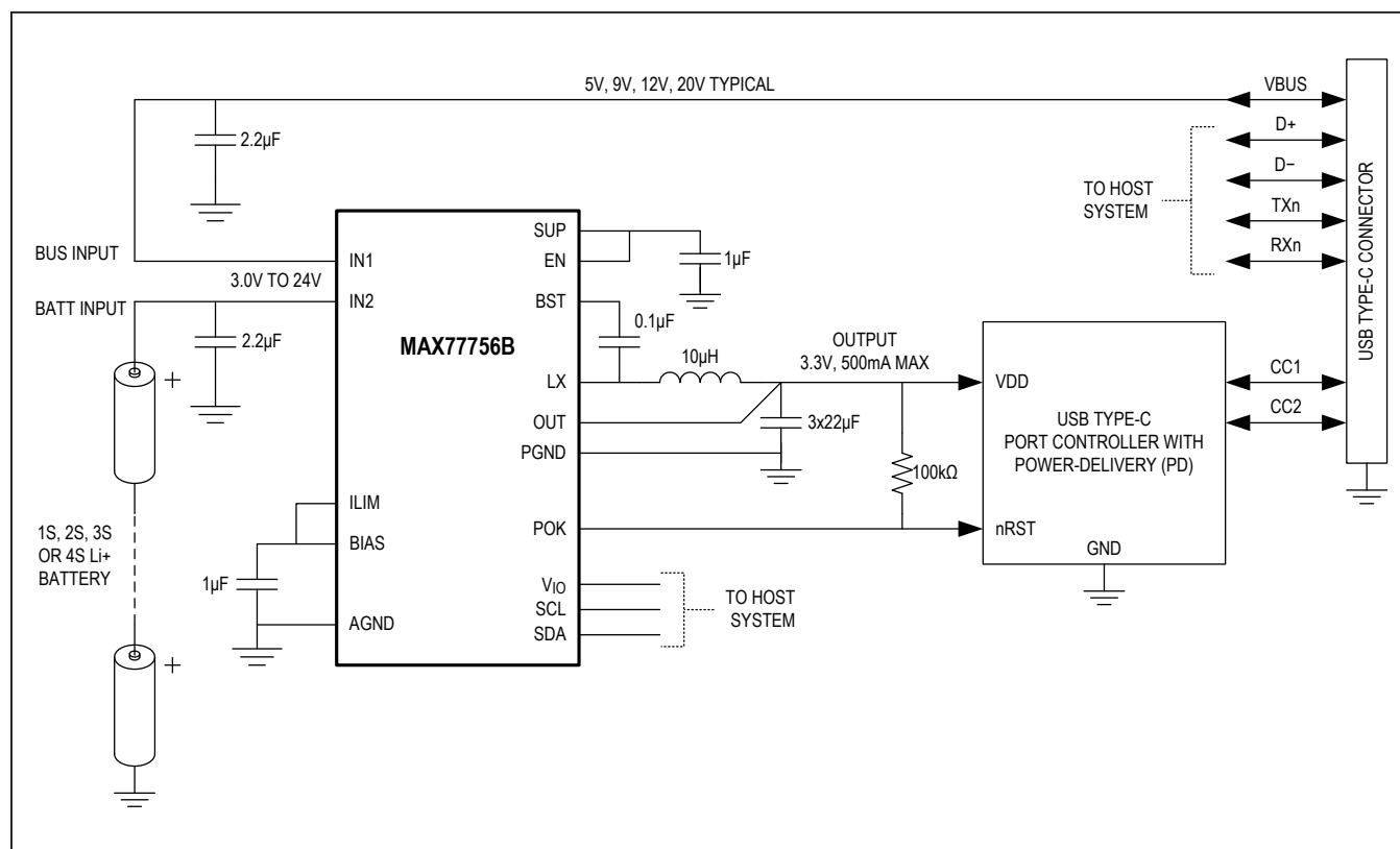
Figure 13. USB Type-C PD Port Controller Power Supply
