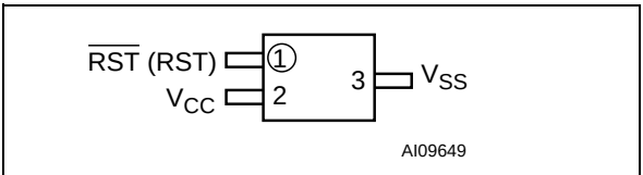
Figure 3. SOT23-3 Connections
