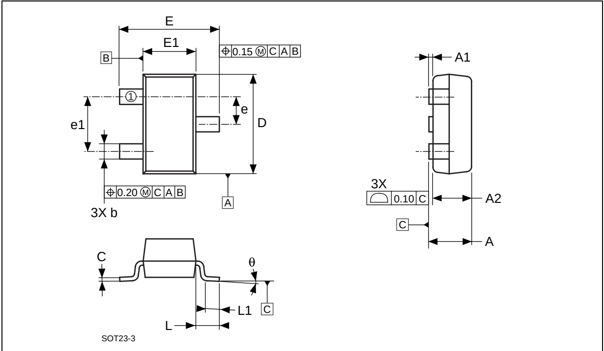
Figure 22. SOT23-3 – 3-lead Small Outline Transistor Package Outline
