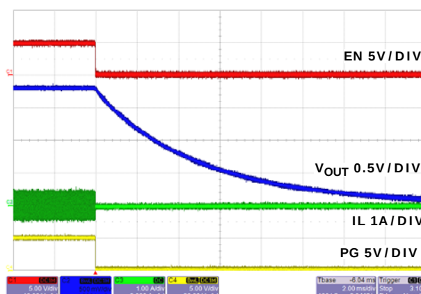
FIGURE 28. SOFT-DISCHARGE SHUTDOWN
