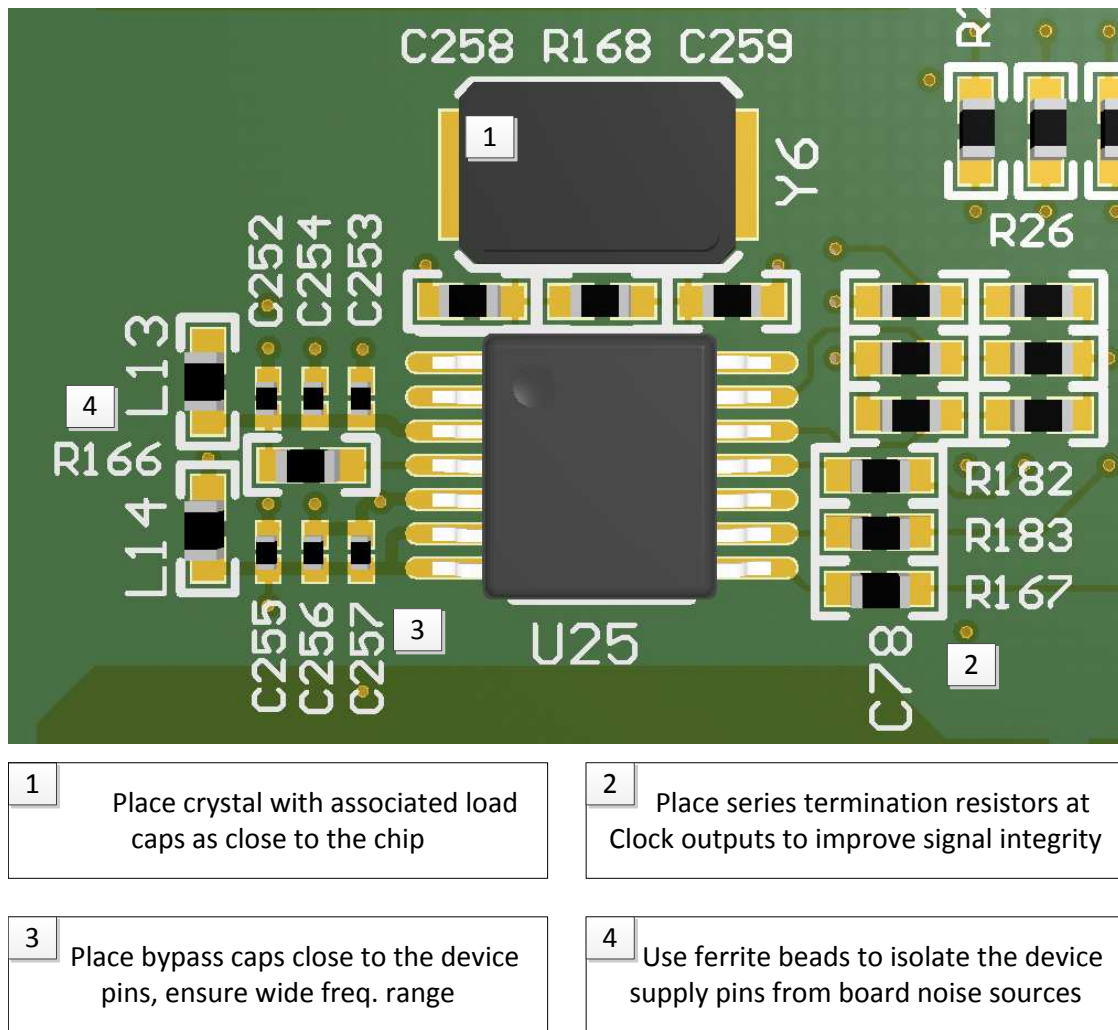
Figure 24. Annotated Layout
