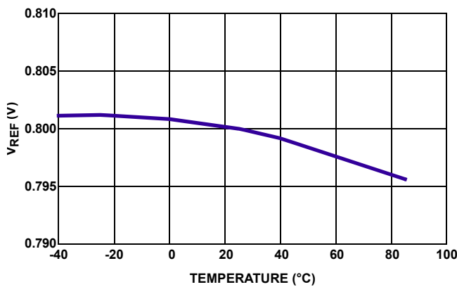
FIGURE 19. V_{REF} vs TEMPERATURE, T_A = -40^{\circ}C TO +85^{\circ}C
