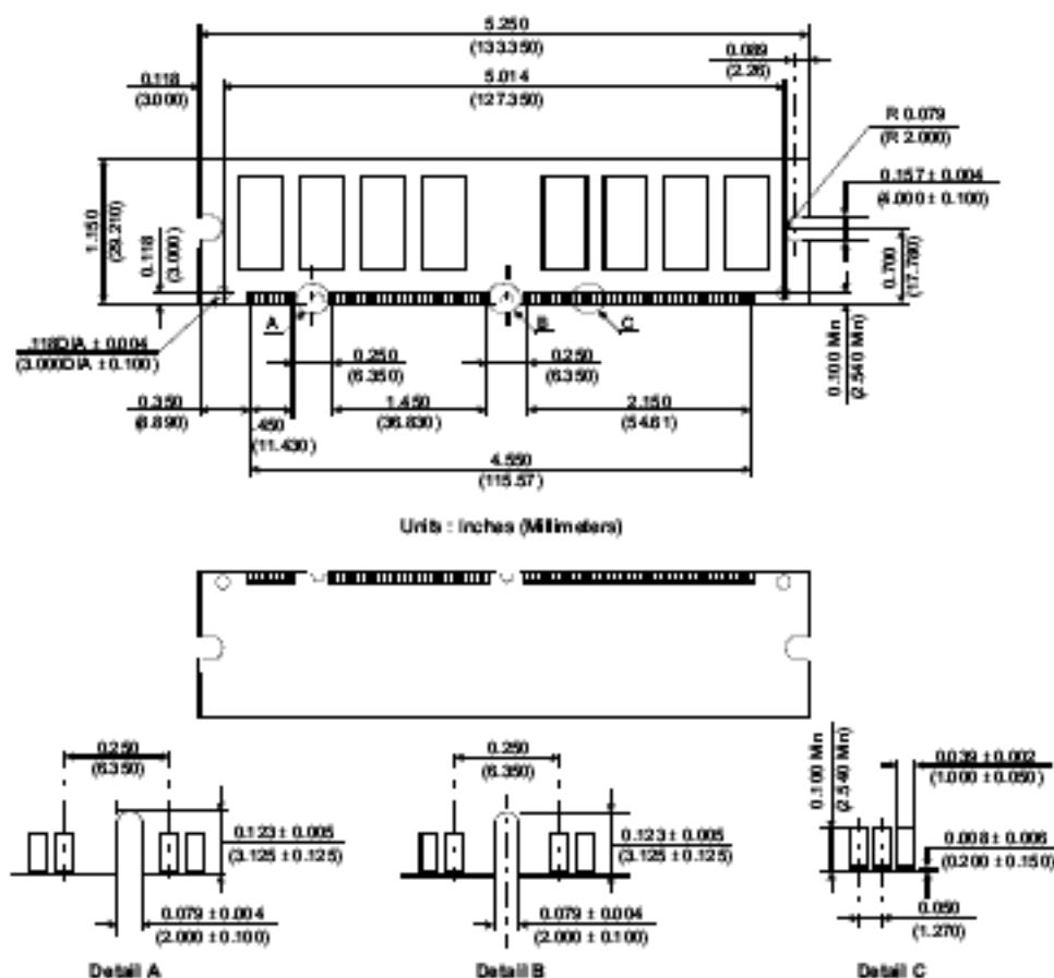
Figure 1: KVR133X64C2/256 168-Pin SDRAM Module
