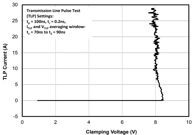
TLP Characteristic
