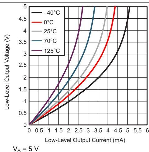
Figure 8. Low-Level Output Voltage vs Low-Level Output Current
