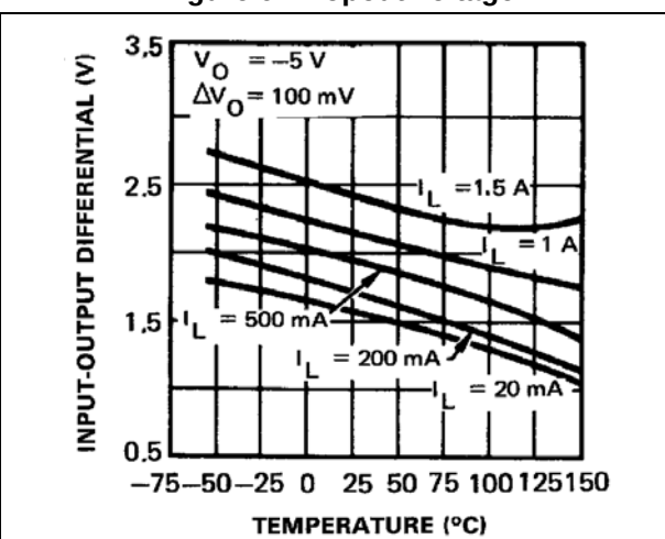
Figure 6. Dropout voltage
