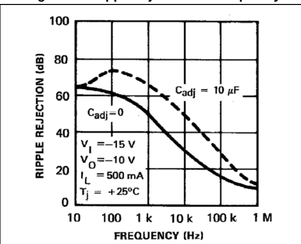
Figure 10. Ripple rejection vs. frequency
