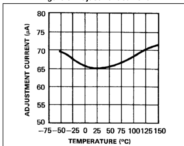
Figure 5. Adjustment current
