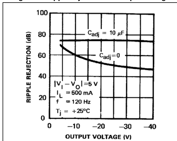
Figure 9. Ripple rejection vs. output voltage
