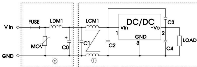
Figure 5 Negative output
