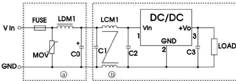
Figure 4 Positive output
