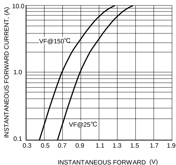
FIG.2-TYPICAL FORWARD CHARACTERISTICS
