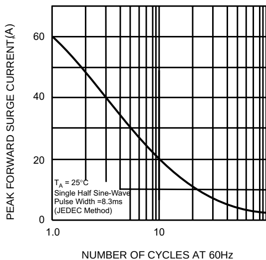
FIG. 3 – MAXIMUM NON-REPEITITIVE SURGE CURRENT
