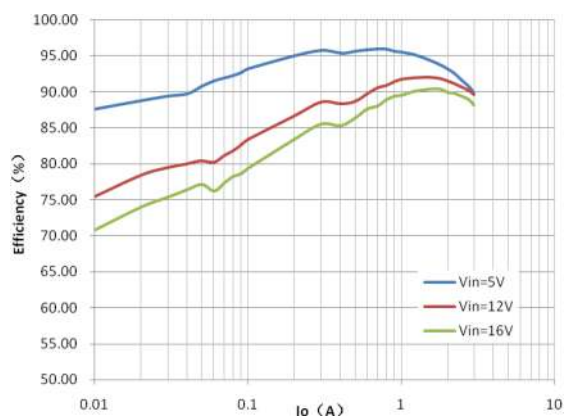
Efficiency @ Vout=3.3V
