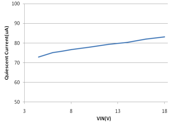
Quiescent Current @ Temperature =25°C
