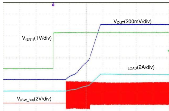
Figure 70. Start-Up With EN1, Forced PWM (3-Phase Output)
