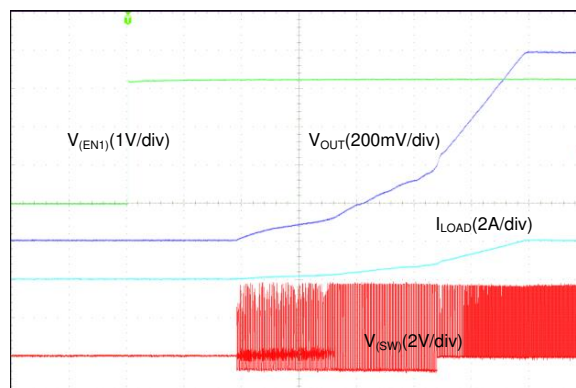
Figure 71. Start-Up With EN1, Forced PWM (2-Phase Output)
