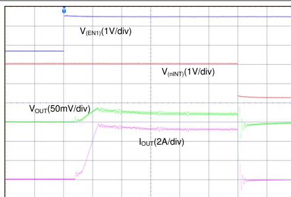
Time (200 \mu\text{s}/\text{div} )
