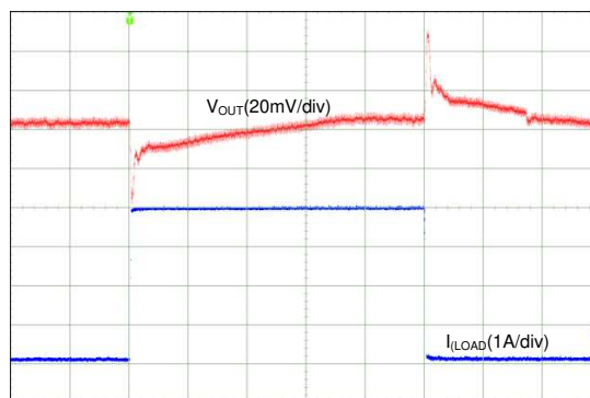
Time (40 \mu\text{s/div} ) I_{OUT} = 0.1\text{ A} \rightarrow 4\text{ A} \rightarrow 0.1\text{ A} T_R = T_F = 1\text{ }\mu\text{s}
