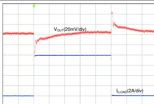
Time (40 \mu\text{s/div} ) I_{OUT} = 0.1\text{ A} \rightarrow 8\text{ A} \rightarrow 0.1\text{ A} T_R = T_F = 1\text{ }\mu\text{s}
