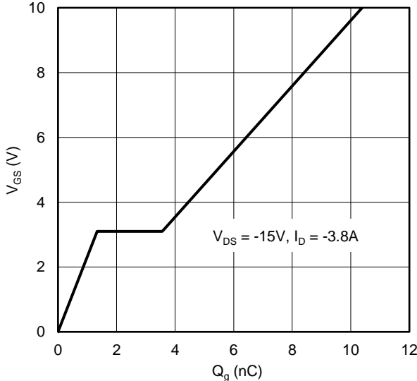
Figure 24. Gate Charge
