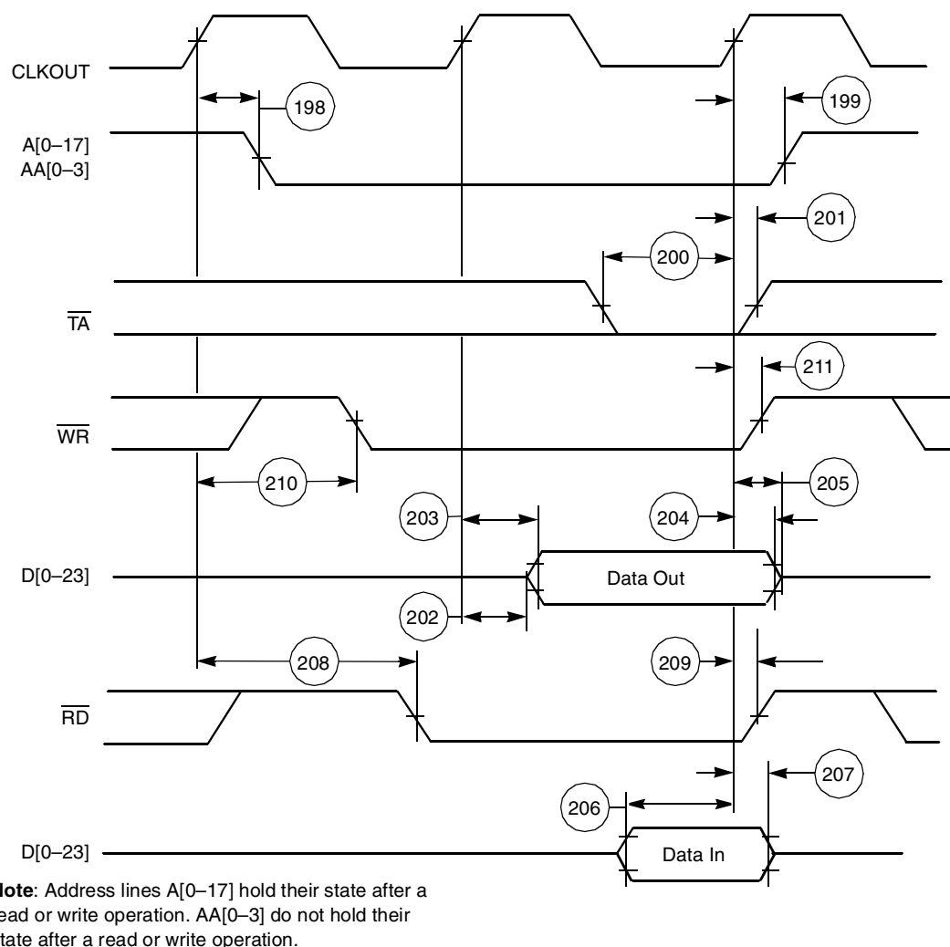
Figure 2-19. Synchronous Bus Timings 1 WS (BCR Controlled)
