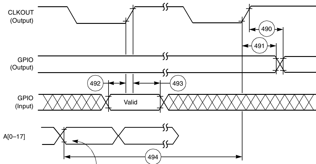
Figure 2-7. GPIO Timing
