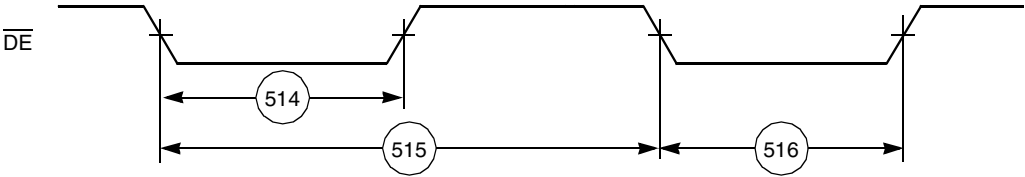
Figure 2-12. OnCE—Debug Request
